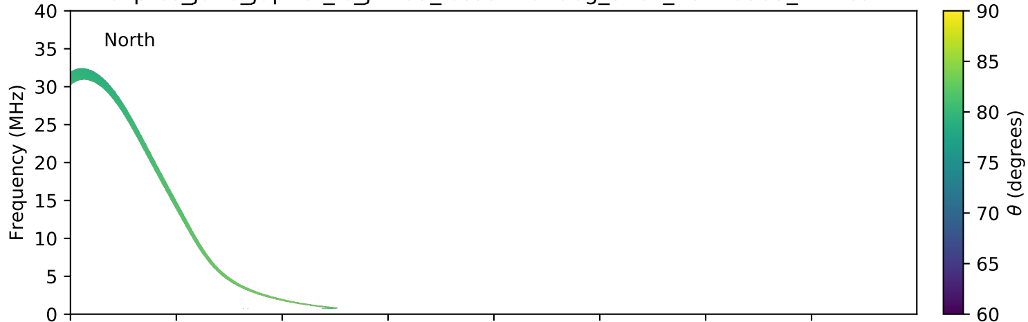
expres_juno_jupiter_io_jrm09_lossc-wid1deg_3kev_20210503_v11.cdf
