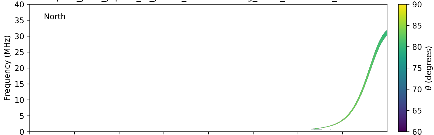
expres_juno_jupiter_io_jrm09_lossc-wid1deg_3kev_20210502_v11.cdf
