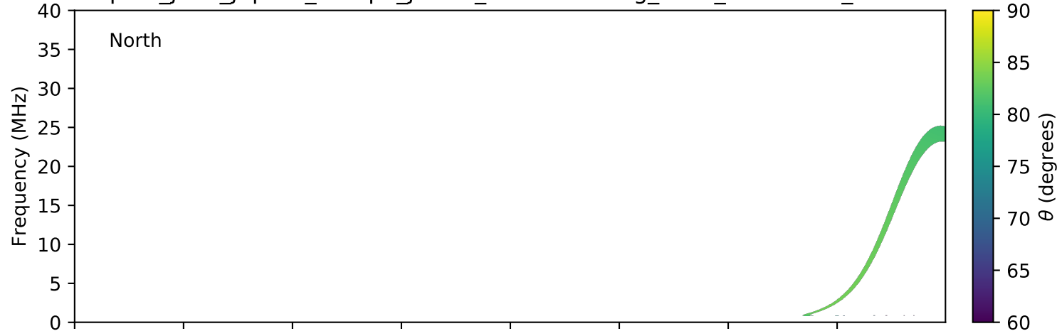
expres_juno_jupiter_europa_jrm09_lossc-wid1deg_3kev_20210526_v11.cdf
