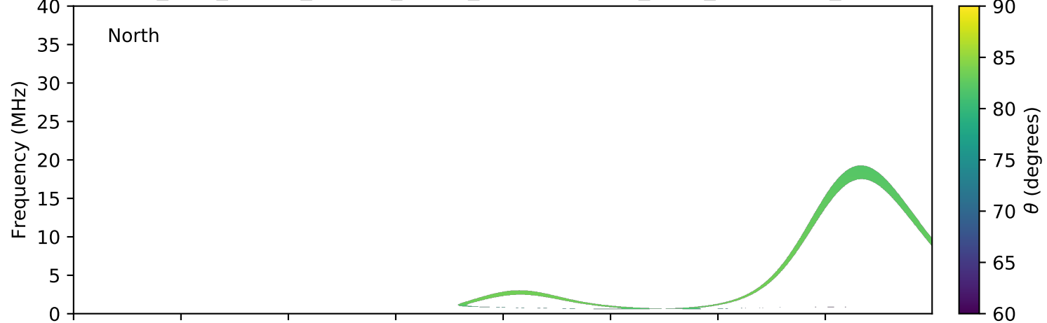
expres_juno_jupiter_europa_jrm09_lossc-wid1deg_3kev_20210505_v11.cdf
