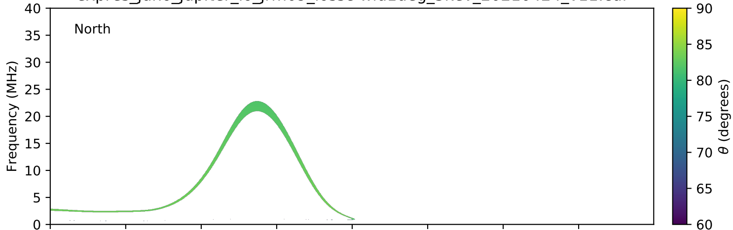
expres_juno_jupiter_io_jrm09_lossc-wid1deg_3kev_20210424_v11.cdf
