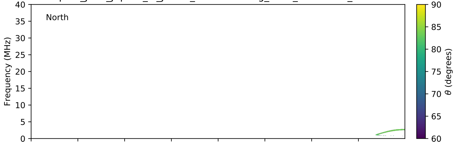
expres_juno_jupiter_io_jrm09_lossc-wid1deg_3kev_20210423_v11.cdf
