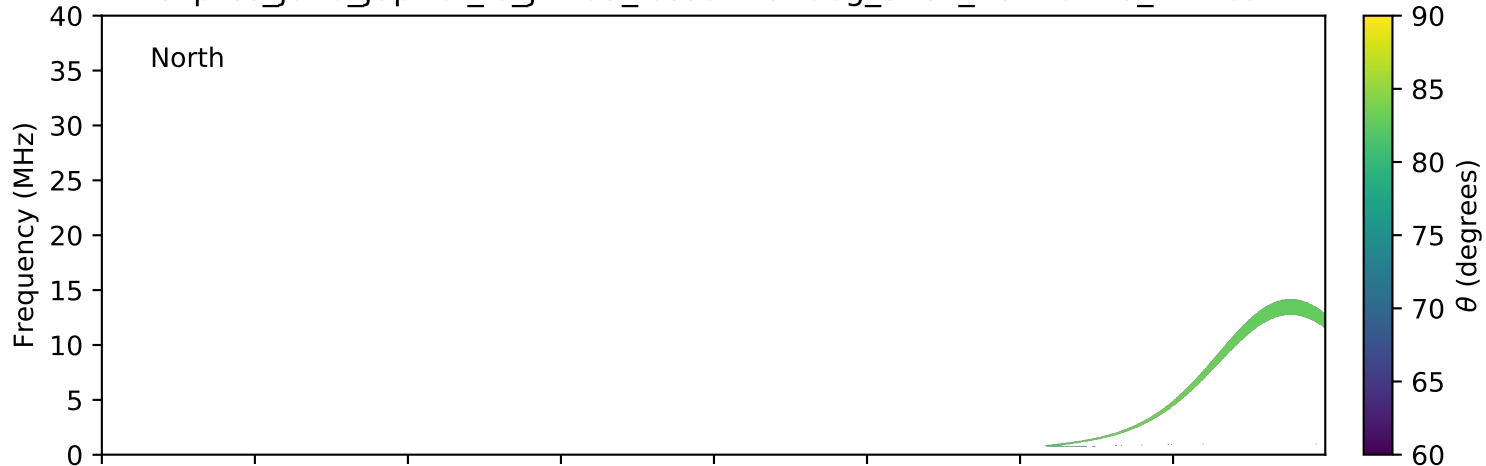
expres_juno_jupiter_io_jrm09_lossc-wid1deg_3kev_20210418_v11.cdf
