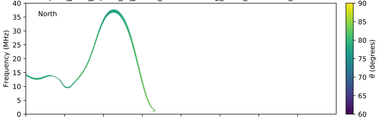
expres_juno_jupiter_io_jrm09_lossc-wid1deg_3kev_20210410_v11.cdf
