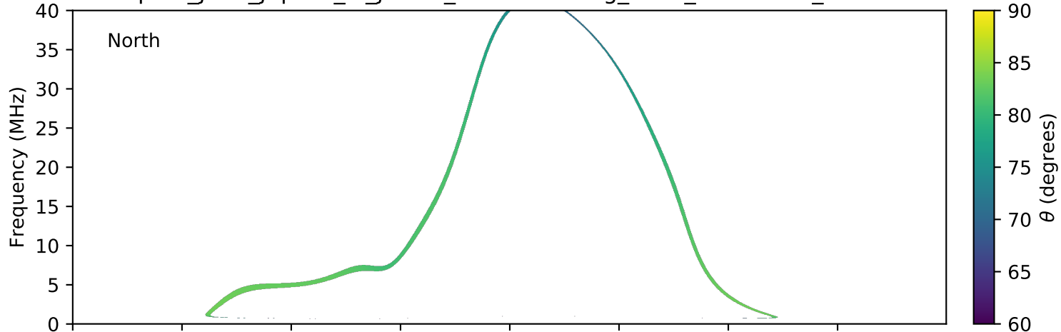
expres_juno_jupiter_io_jrm09_lossc-wid1deg_3kev_20210406_v11.cdf
