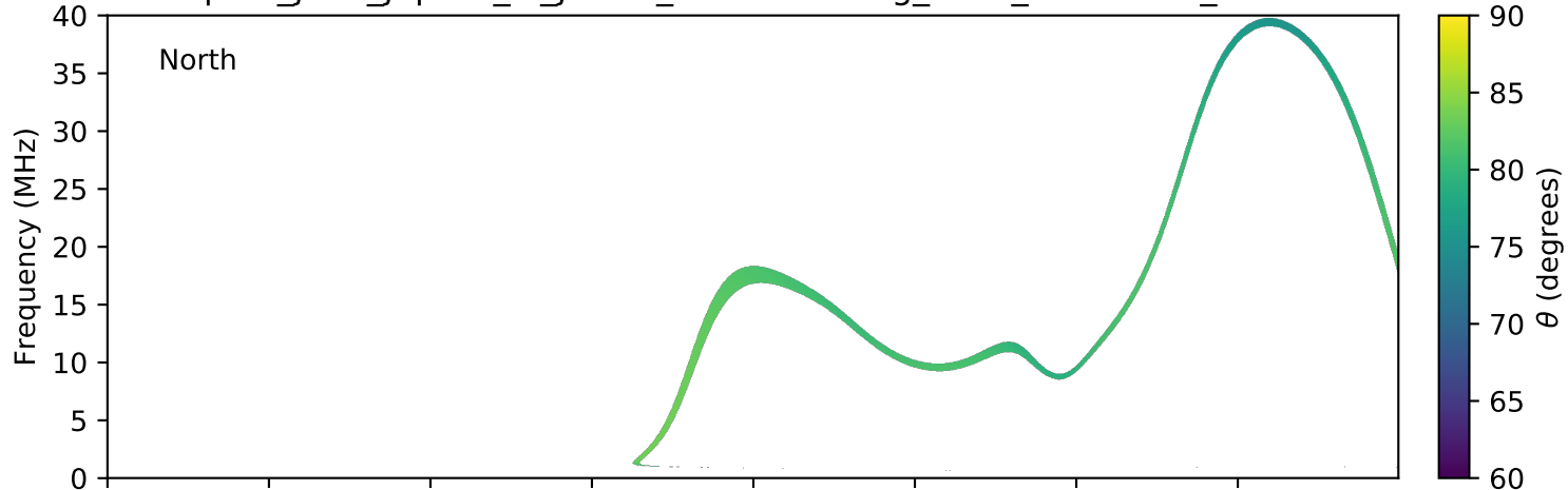
expres_juno_jupiter_io_jrm09_lossc-wid1deg_3kev_20210404_v11.cdf
