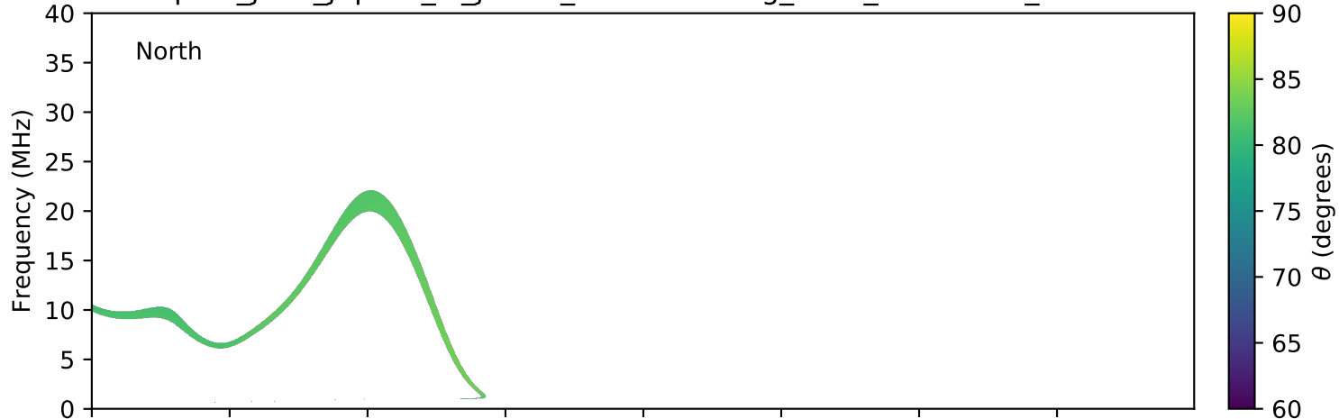
expres_juno_jupiter_io_jrm09_lossc-wid1deg_3kev_20210403_v11.cdf
