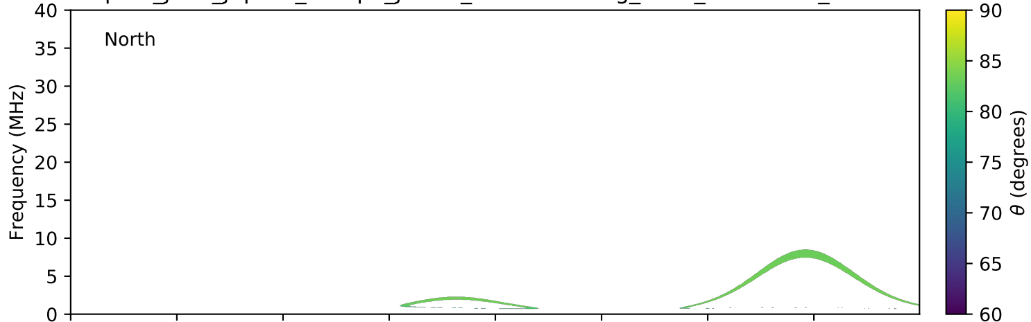
expres_juno_jupiter_europa_jrm09_lossc-wid1deg_3kev_20210421_v11.cdf
