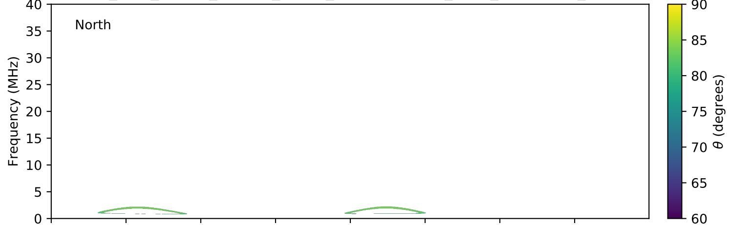
expres_juno_jupiter_europa_jrm09_lossc-wid1deg_3kev_20210418_v11.cdf
