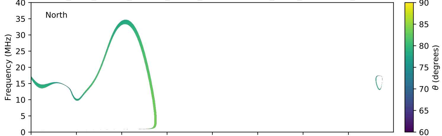
expres_juno_jupiter_europa_jrm09_lossc-wid1deg_3kev_20210415_v11.cdf
