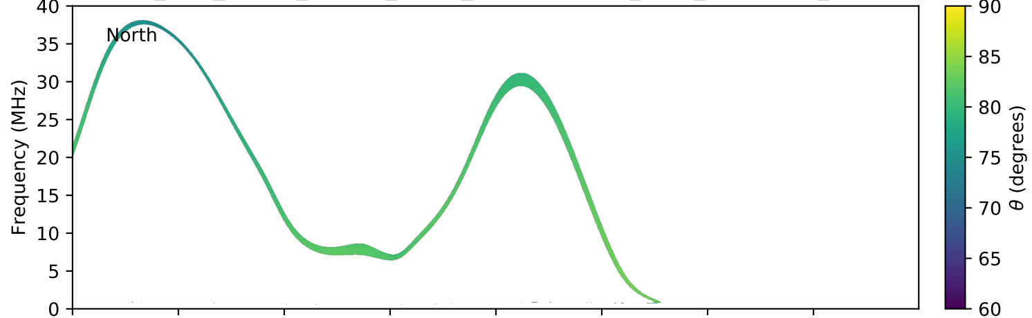
expres_juno_jupiter_europa_jrm09_lossc-wid1deg_3kev_20210411_v11.cdf
