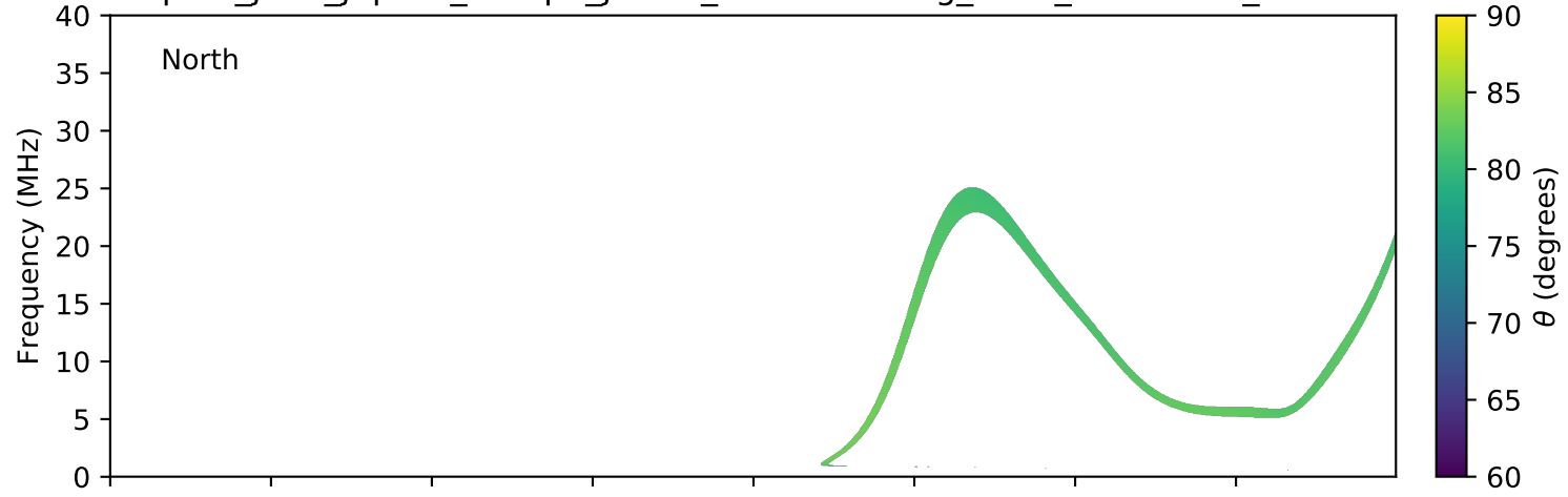
expres_juno_jupiter_europa_jrm09_lossc-wid1deg_3kev_20210410_v11.cdf
