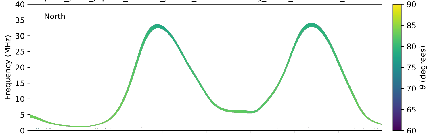
expres_juno_jupiter_europa_jrm09_lossc-wid1deg_3kev_20210407_v11.cdf
