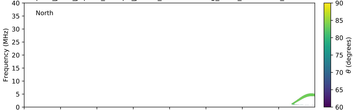
expres_juno_jupiter_europa_jrm09_lossc-wid1deg_3kev_20210406_v11.cdf
