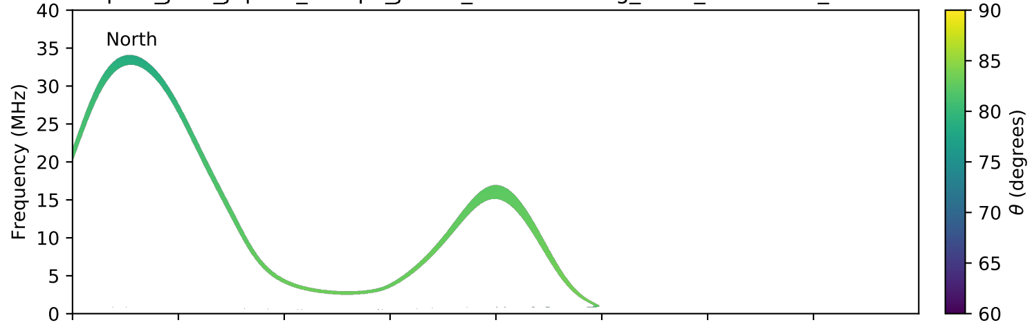
expres_juno_jupiter_europa_jrm09_lossc-wid1deg_3kev_20210404_v11.cdf
