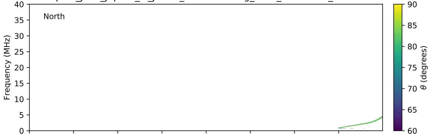
expres_juno_jupiter_io_jrm09_lossc-wid1deg_3kev_20210331_v11.cdf
