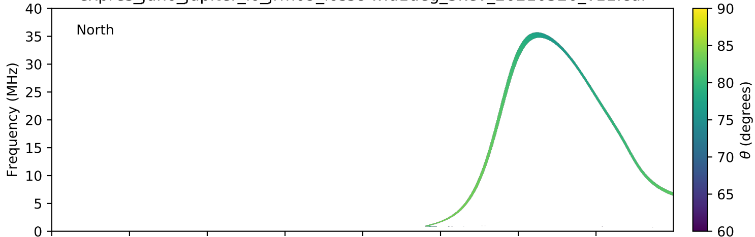
expres_juno_jupiter_io_jrm09_lossc-wid1deg_3kev_20210326_v11.cdf
