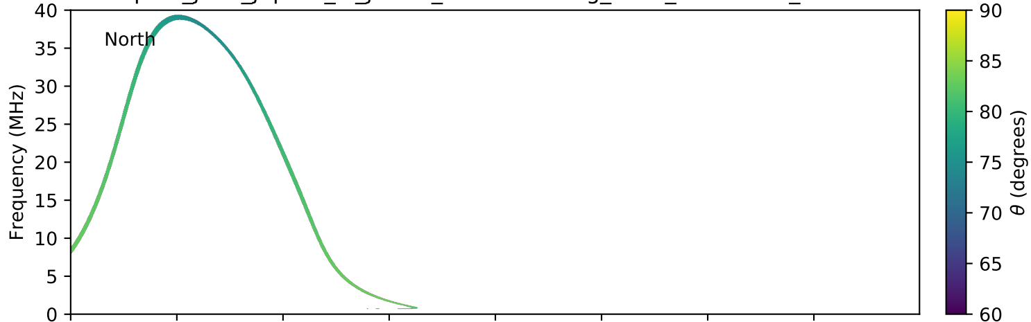
expres_juno_jupiter_io_jrm09_lossc-wid1deg_3kev_20210325_v11.cdf
