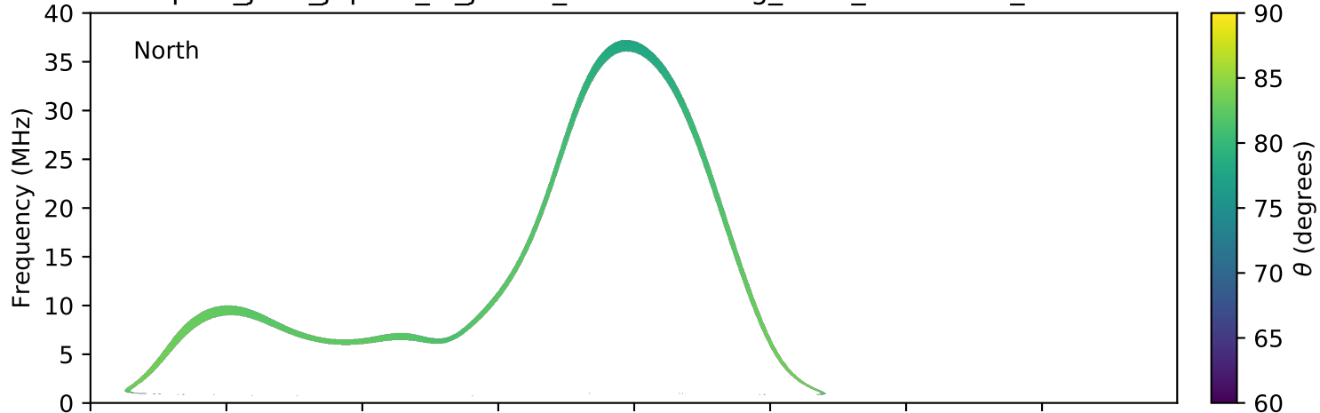
expres_juno_jupiter_io_jrm09_lossc-wid1deg_3kev_20210323_v11.cdf
