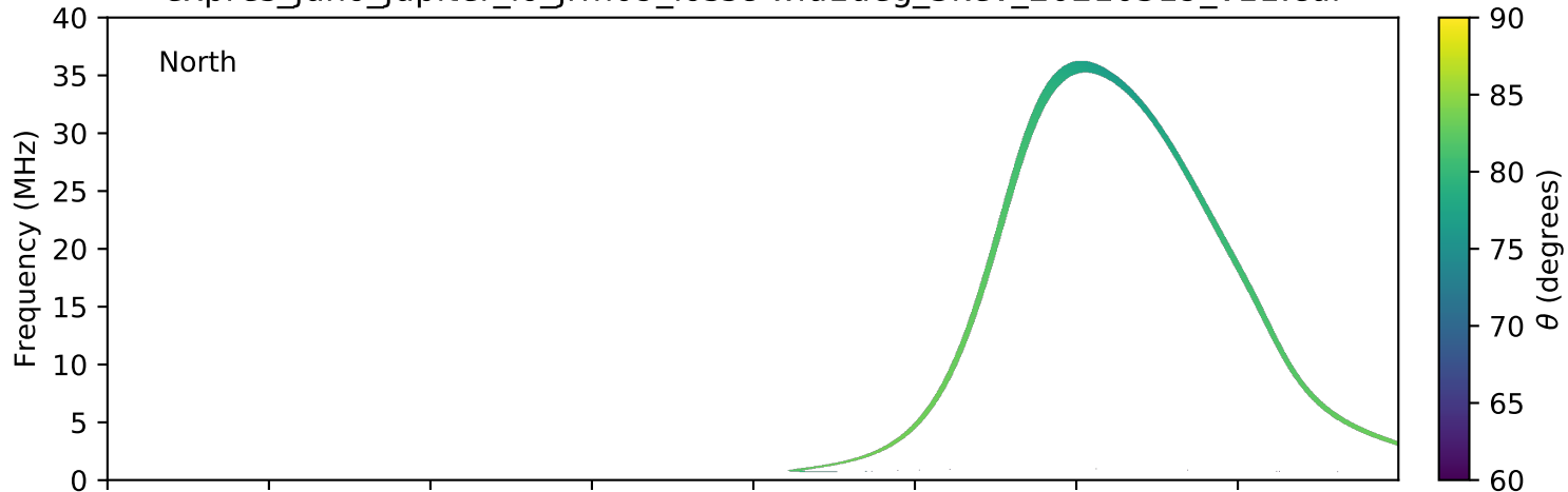
expres_juno_jupiter_io_jrm09_lossc-wid1deg_3kev_20210319_v11.cdf
