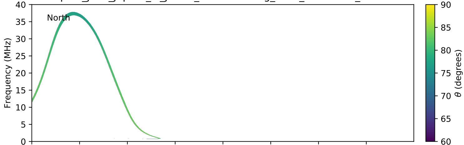
expres_juno_jupiter_io_jrm09_lossc-wid1deg_3kev_20210318_v11.cdf
