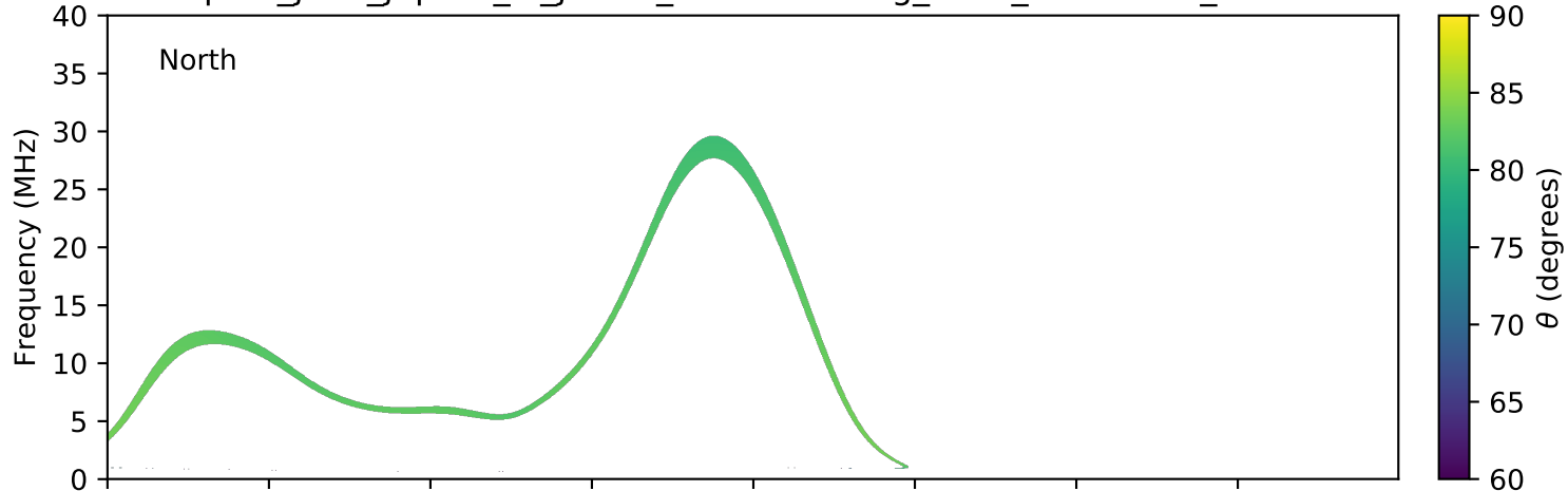
expres_juno_jupiter_io_jrm09_lossc-wid1deg_3kev_20210316_v11.cdf
