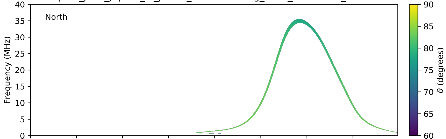
expres_juno_jupiter_io_jrm09_lossc-wid1deg_3kev_20210312_v11.cdf
