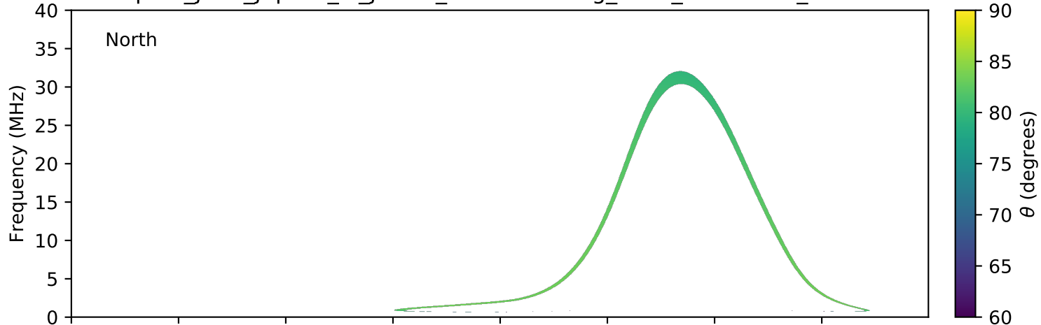
expres_juno_jupiter_io_jrm09_lossc-wid1deg_3kev_20210305_v11.cdf
