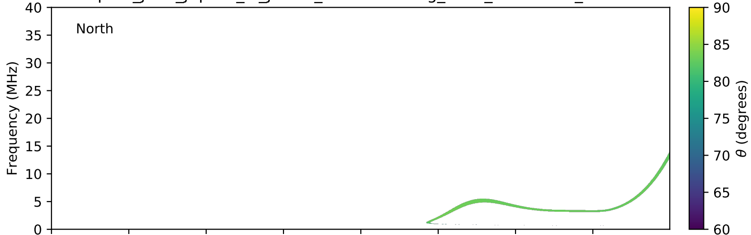
expres_juno_jupiter_io_jrm09_lossc-wid1deg_3kev_20210303_v11.cdf
