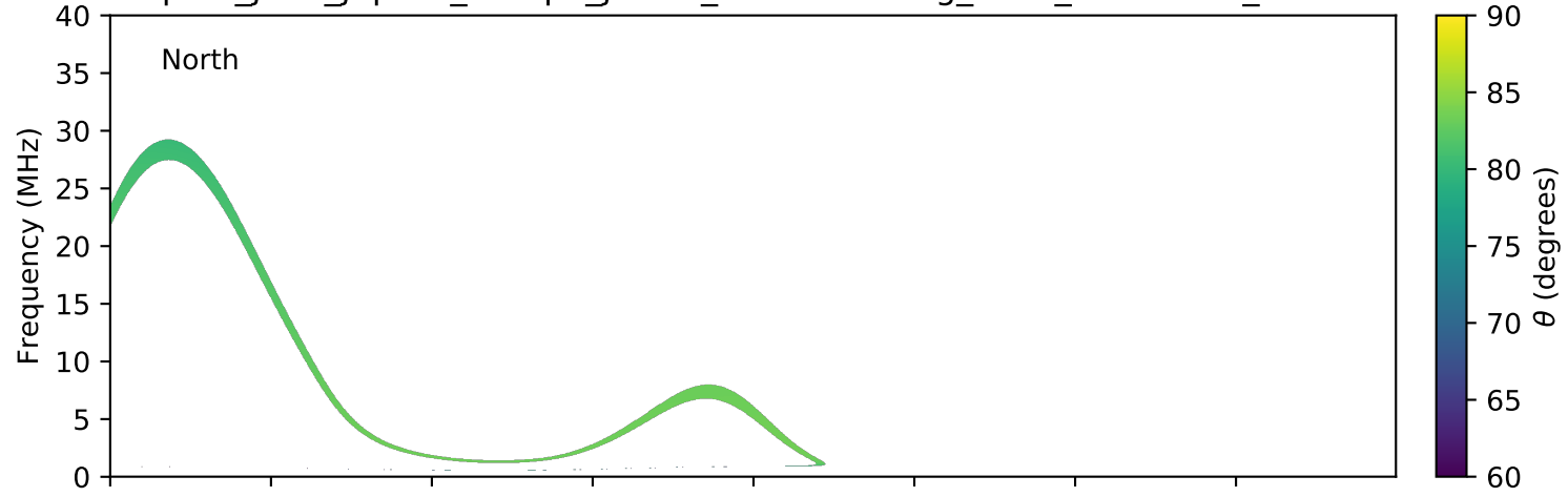
expres_juno_jupiter_europa_jrm09_lossc-wid1deg_3kev_20210328_v11.cdf
