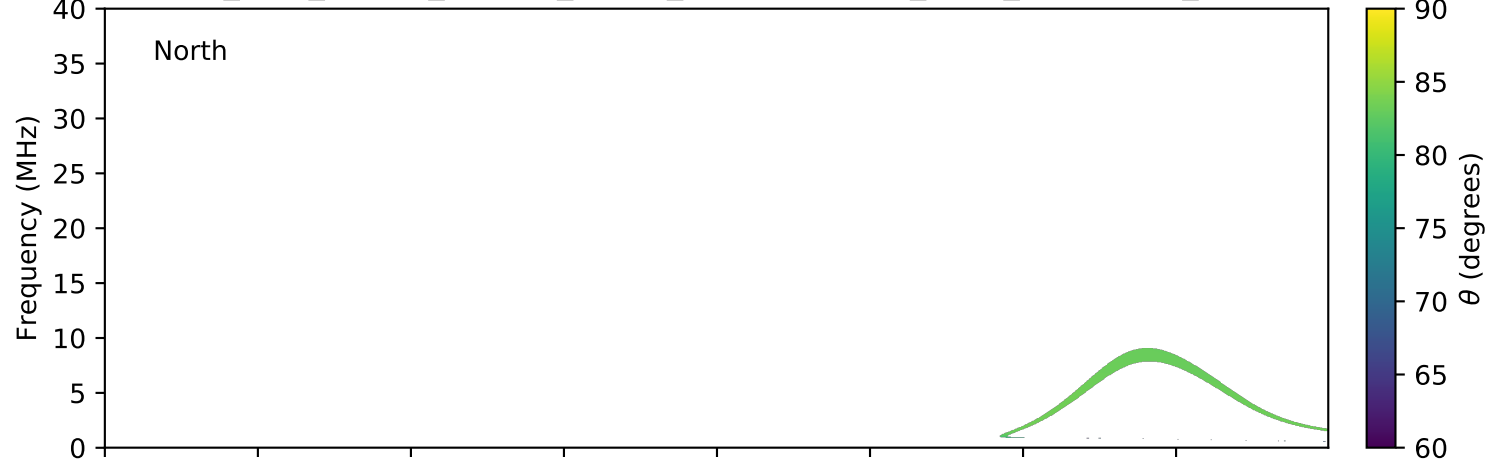
expres_juno_jupiter_europa_jrm09_lossc-wid1deg_3kev_20210309_v11.cdf
