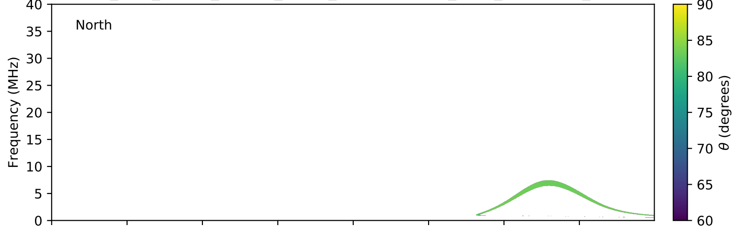
expres_juno_jupiter_europa_jrm09_lossc-wid1deg_3kev_20210302_v11.cdf
