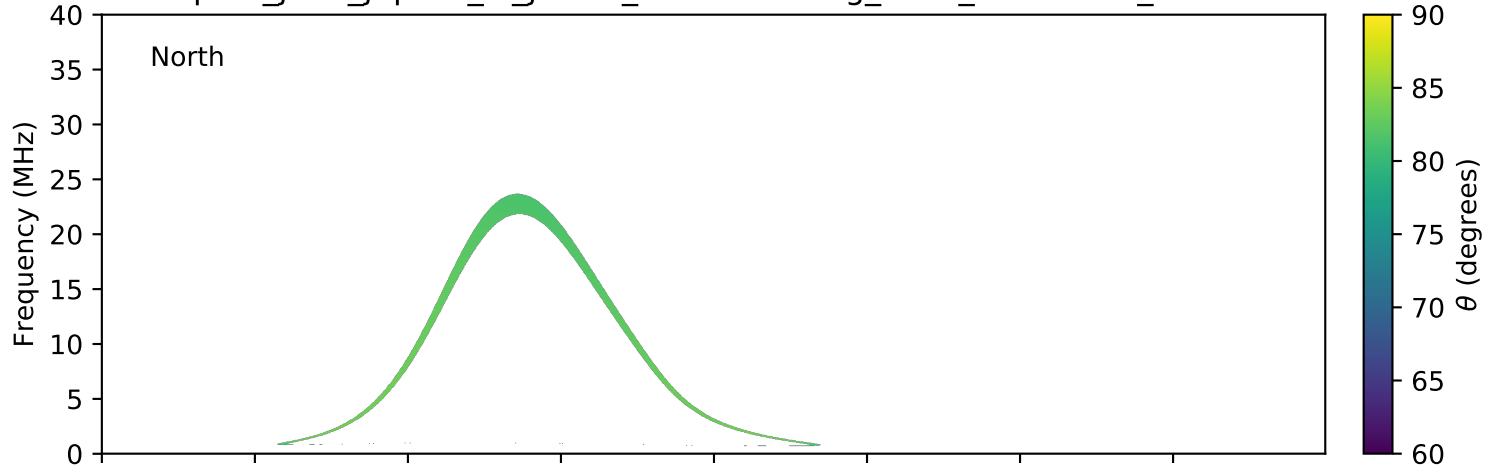
expres_juno_jupiter_io_jrm09_lossc-wid1deg_3kev_20210228_v11.cdf
