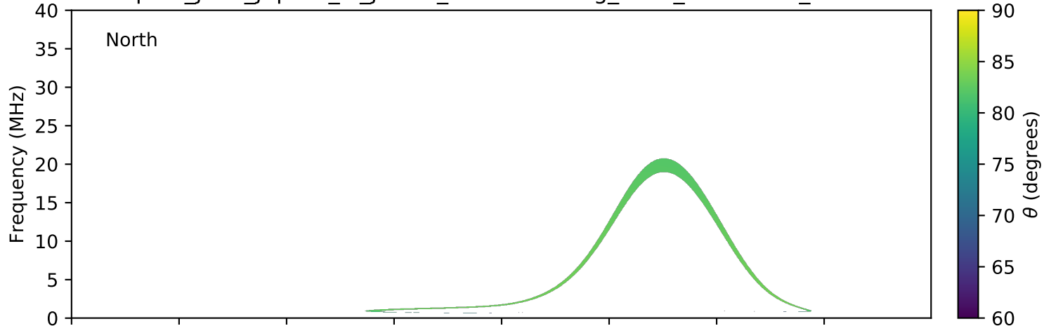
expres_juno_jupiter_io_jrm09_lossc-wid1deg_3kev_20210226_v11.cdf
