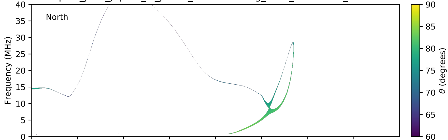
expres_juno_jupiter_io_jrm09_lossc-wid1deg_3kev_20210221_v11.cdf
