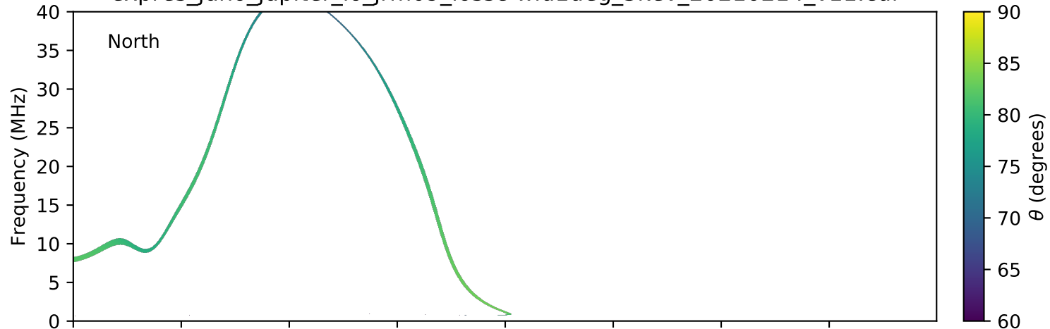
expres_juno_jupiter_io_jrm09_lossc-wid1deg_3kev_20210214_v11.cdf
