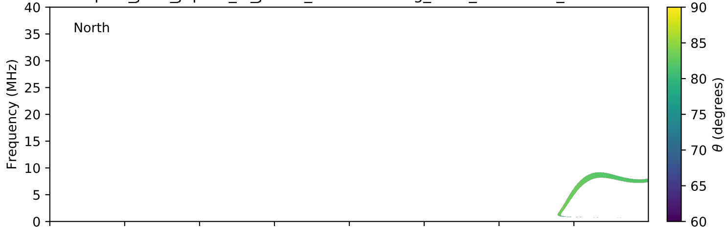
expres_juno_jupiter_io_jrm09_lossc-wid1deg_3kev_20210213_v11.cdf
