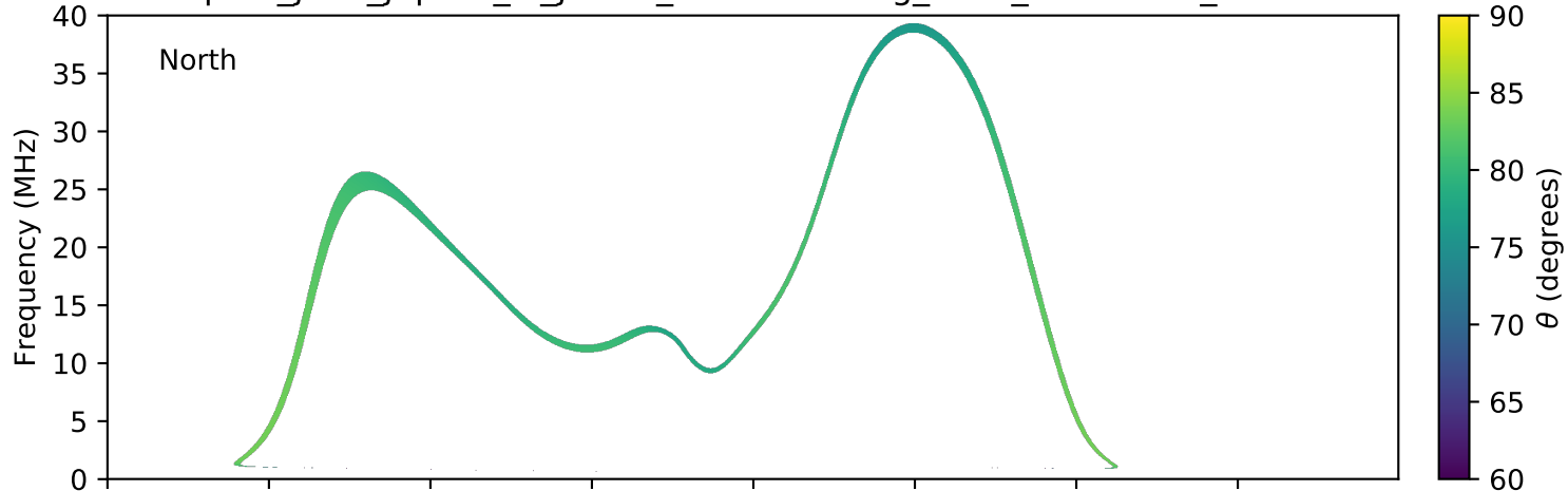
expres_juno_jupiter_io_jrm09_lossc-wid1deg_3kev_20210212_v11.cdf
