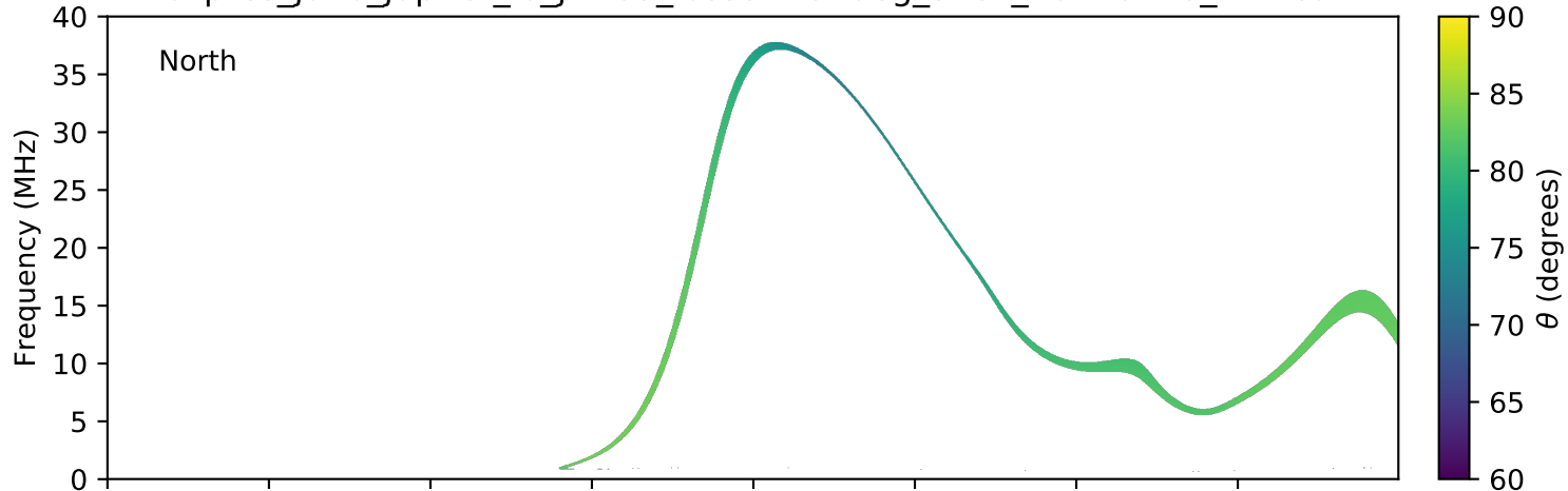
expres_juno_jupiter_io_jrm09_lossc-wid1deg_3kev_20210210_v11.cdf
