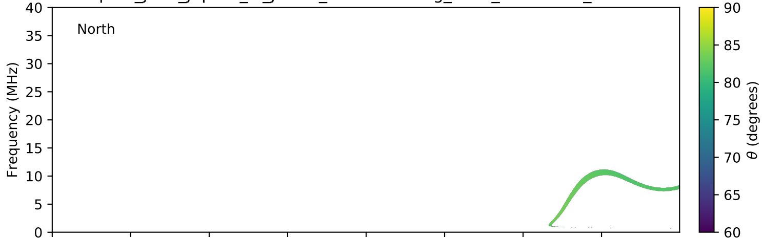
expres_juno_jupiter_io_jrm09_lossc-wid1deg_3kev_20210206_v11.cdf
