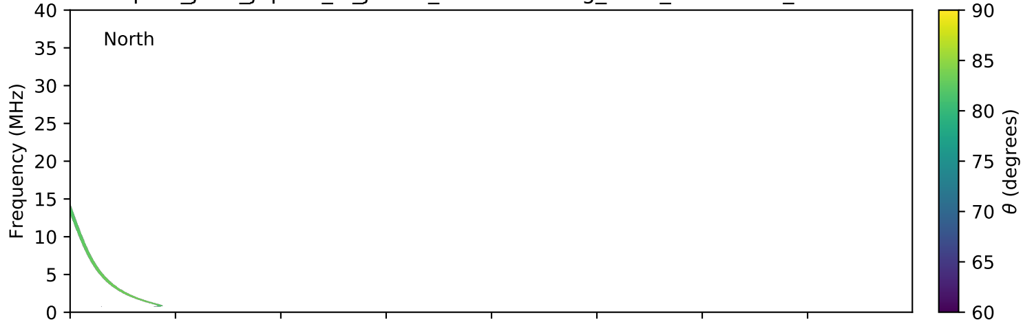
expres_juno_jupiter_io_jrm09_lossc-wid1deg_3kev_20210202_v11.cdf
