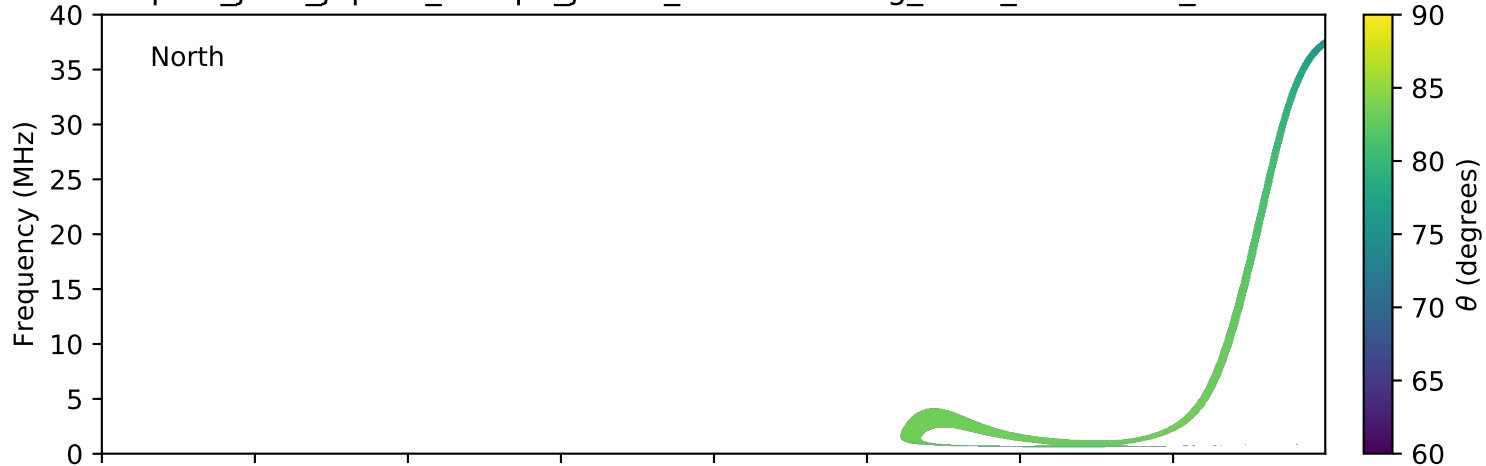
expres_juno_jupiter_europa_jrm09_lossc-wid1deg_3kev_20210219_v11.cdf
