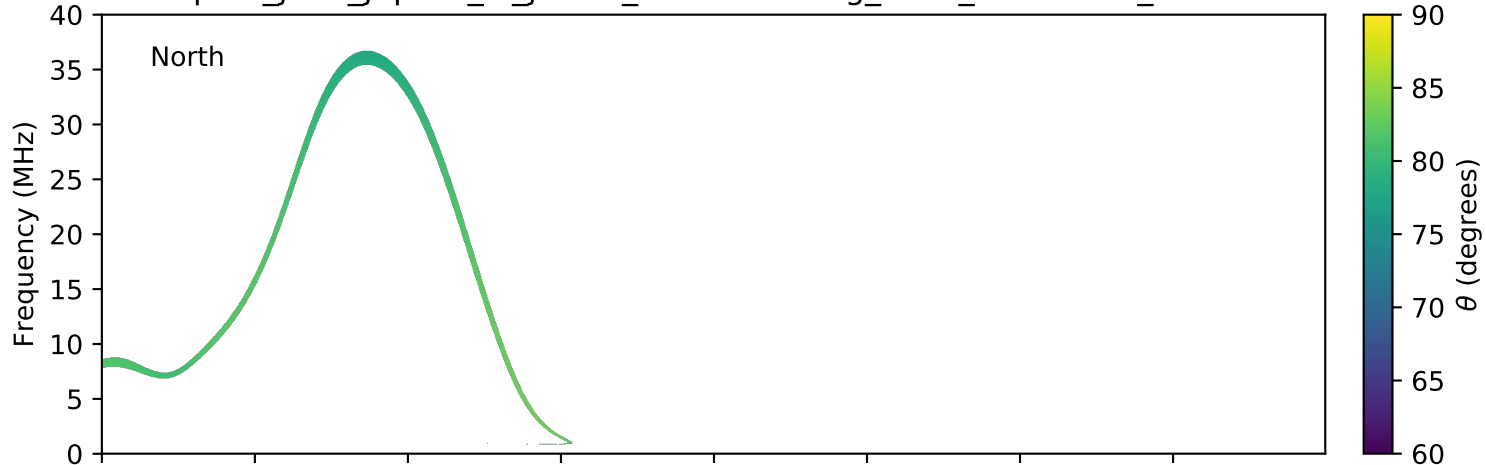
expres_juno_jupiter_io_jrm09_lossc-wid1deg_3kev_20210131_v11.cdf
