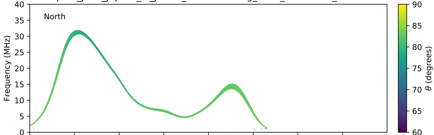
expres_juno_jupiter_io_jrm09_lossc-wid1deg_3kev_20210129_v11.cdf
