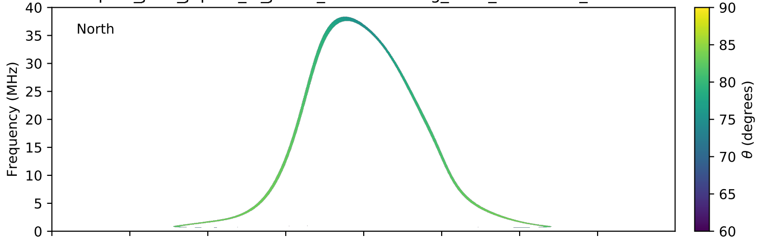
expres_juno_jupiter_io_jrm09_lossc-wid1deg_3kev_20210127_v11.cdf
