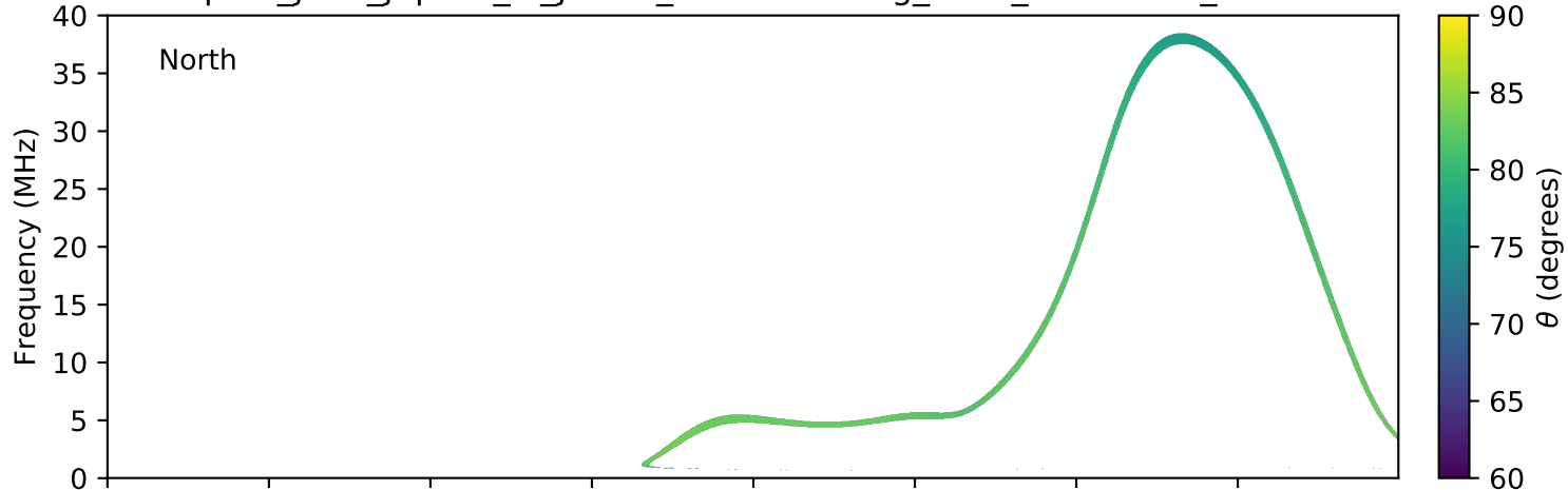
expres_juno_jupiter_io_jrm09_lossc-wid1deg_3kev_20210125_v11.cdf
