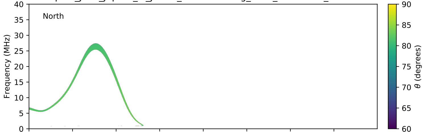
expres_juno_jupiter_io_jrm09_lossc-wid1deg_3kev_20210124_v11.cdf
