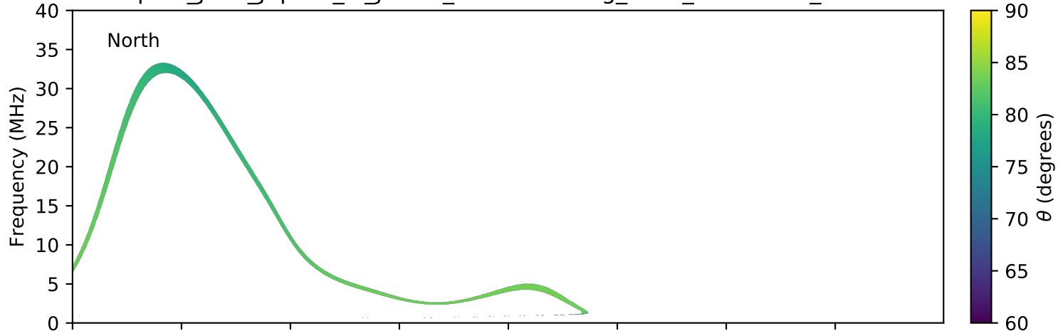
expres_juno_jupiter_io_jrm09_lossc-wid1deg_3kev_20210122_v11.cdf
