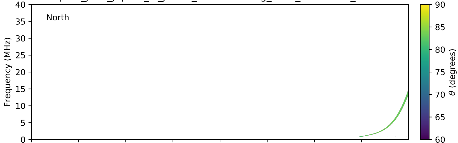
expres_juno_jupiter_io_jrm09_lossc-wid1deg_3kev_20210114_v11.cdf
