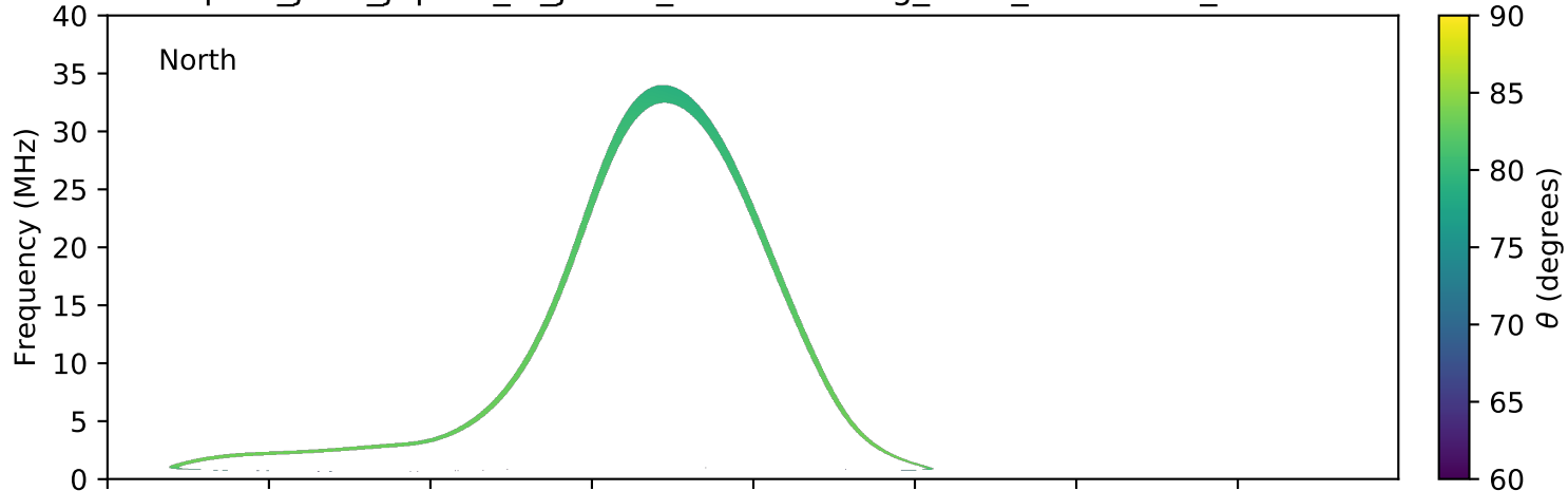
expres_juno_jupiter_io_jrm09_lossc-wid1deg_3kev_20210113_v11.cdf
